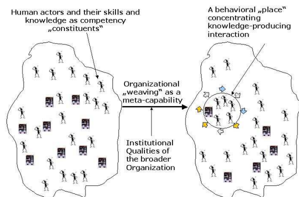
Fig. 2. Conceptual framework [33]
